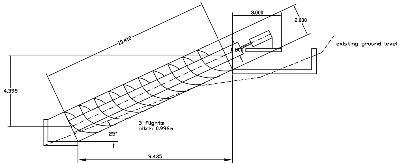
SECTION A-A THROUGH SCREW
