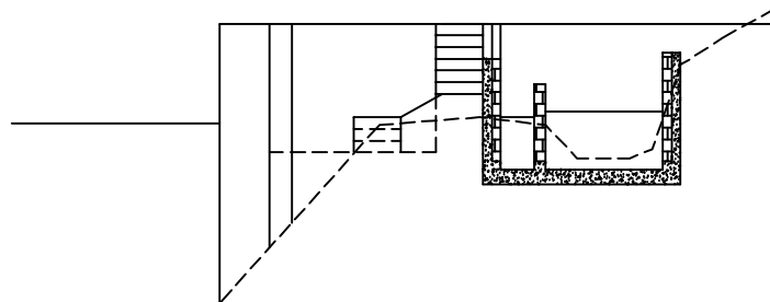
SECTION B-B THROUGH APPROACH CHANNELS
