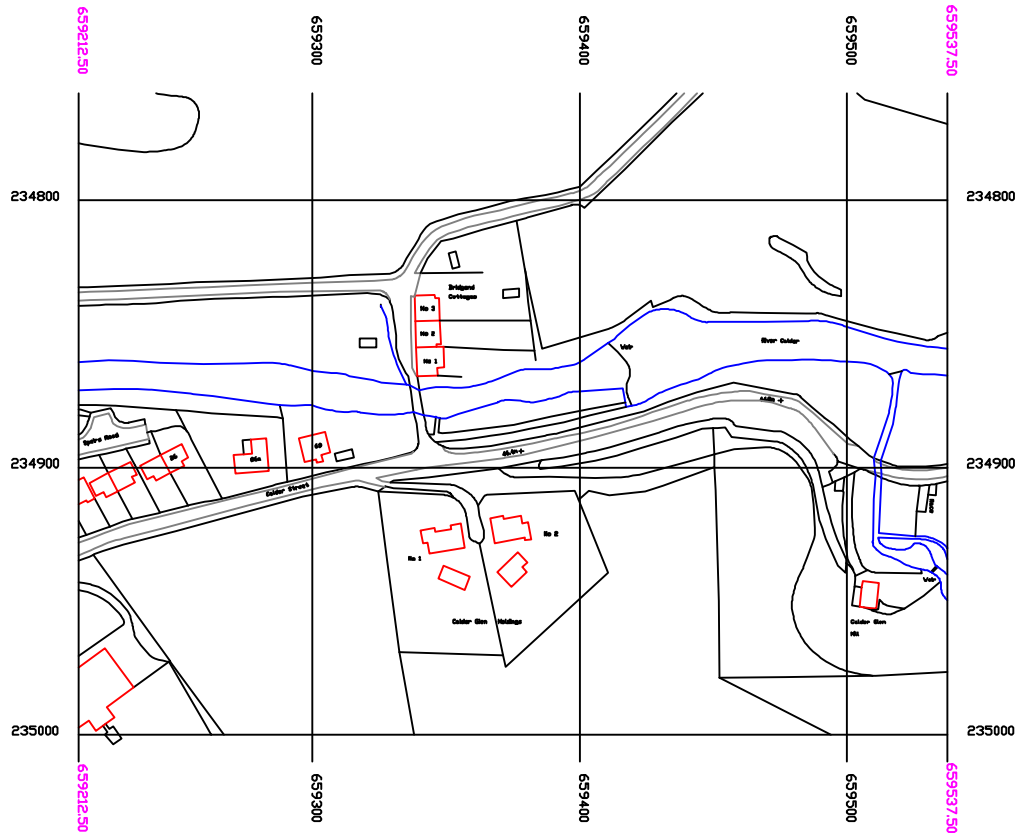
GENERAL LAYOUT scale 1/500
